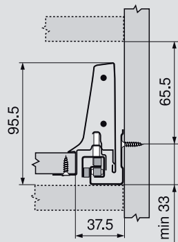
Space requirements in cabinet
