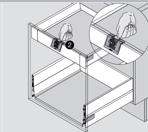
Release
