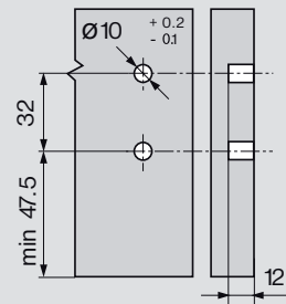
Drilling dimensions for INSERTA and knock-in front
