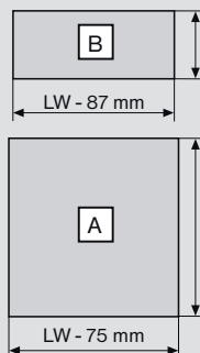
Cutting dim. for 16 mm chipboard
